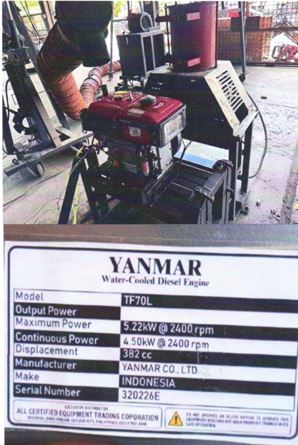
Figure 1. Engine test set up and nameplate of the YANMAR TF70L Diesel Engine.
